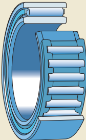
NAO
